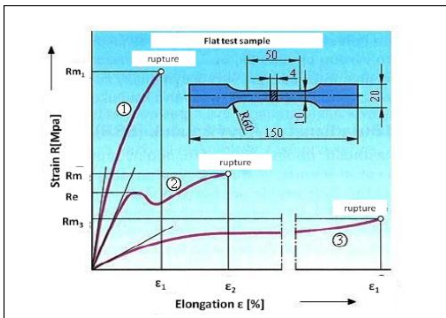
Fig. 2 Diagrams tensile test different types of plastics
