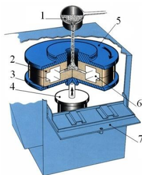
Fig. 1 Scheme of the process of centrifugal casting method Tekcast [3], 1 - molten metal or plastic in a liquid state, 2 - silicone form 3 - bottom plate, 4 - air cylinder, 5 - top plate, 6 - shave of mold cavity, 7 - door
